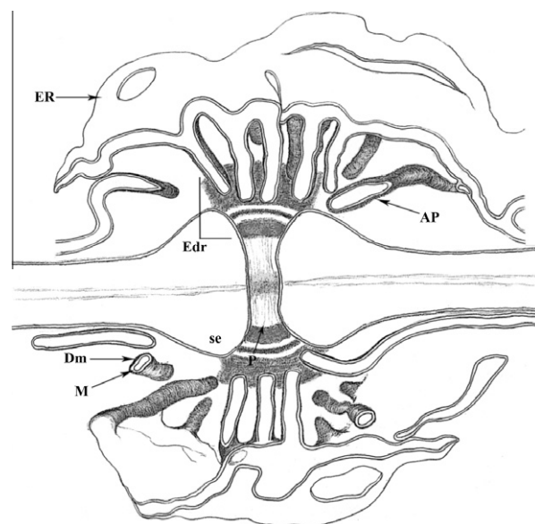
Fig. 3. Three-dimensional reconstruction of the septal pore apparatus in Wallemia sebi . AP, adseptal finger-like processes; Dm, electron-dense material; Edr, electron dense region; ER, endoplasmic reticulum; M, membrane; P, septal pore; se, septal pore swelling. Copyright Regents of the University of Minnesota and David McLaughlin.
